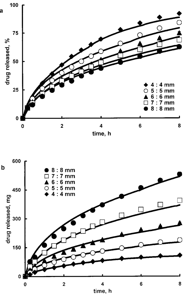
Fig. 7. Effect of the initial tablet size on the release patterns of chlorpheniramine maleate from HPMC K15M-based matrix tablets in 0.1 M HCl: (a) relative amount of drug released; and (b) absolute amount of drug released vs. time (curves: predicted values, symbols: independent experimental data).
